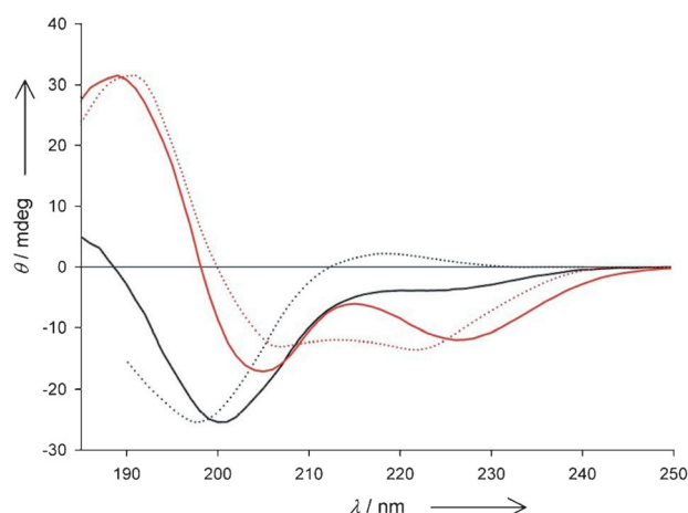
Figure 5. Far-UV CD spectra of peptides P-1 (black solid line) and P-2 (red solid line) in comparison to the spectra of random-coiled peptides (black dotted line) and 100 % \alpha -helical poly-L-glutamic acid at low pH (red dotted line). The pairs of similar spectra were scaled to their maximum Cotton effects.
